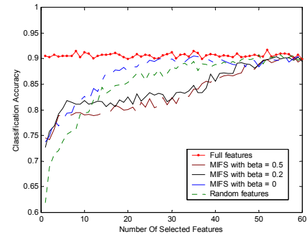
Figure 6: Classification Performance
