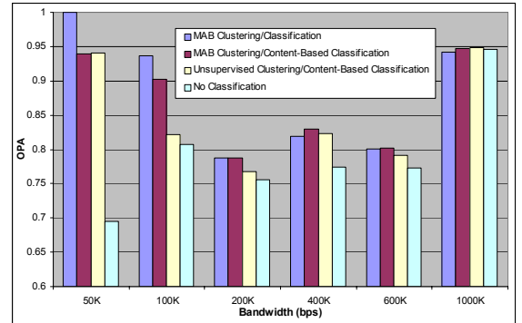
Figure 8: Operation prediction accuracy
