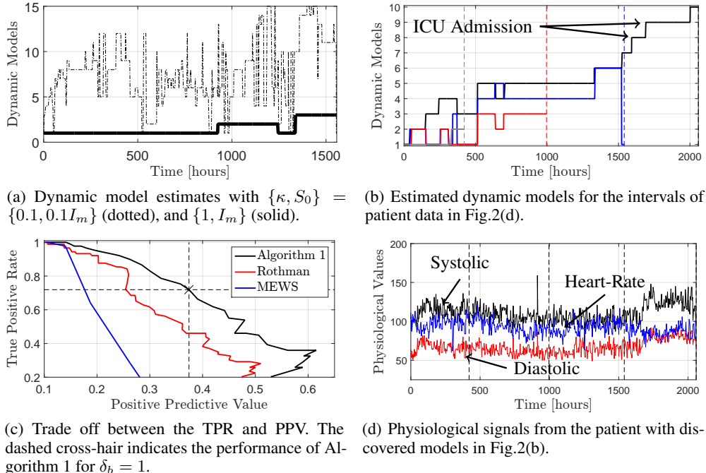
Figure 2: Dynamic model discovery and performance of Algorithm 1.
