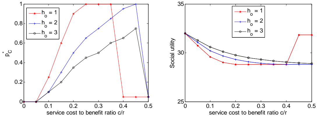
Figure 4. The optimal fraction of altruistic peers p_C^* and the corresponding social utility
