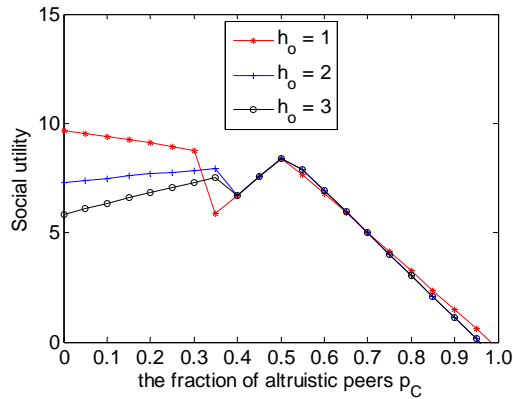
Figure 3. Social utility of all peers against p_C
