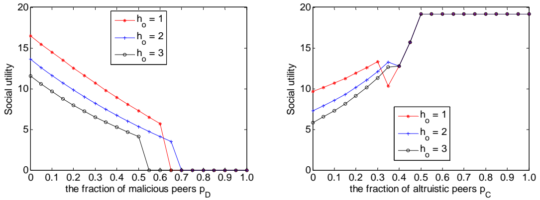
Figure 2. Average utility of reciprocal peers against p_D and p_C
