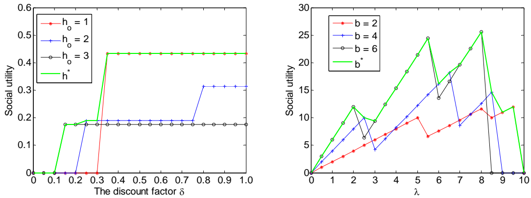
Figure 6. The protocols' performance against \beta and \lambda
