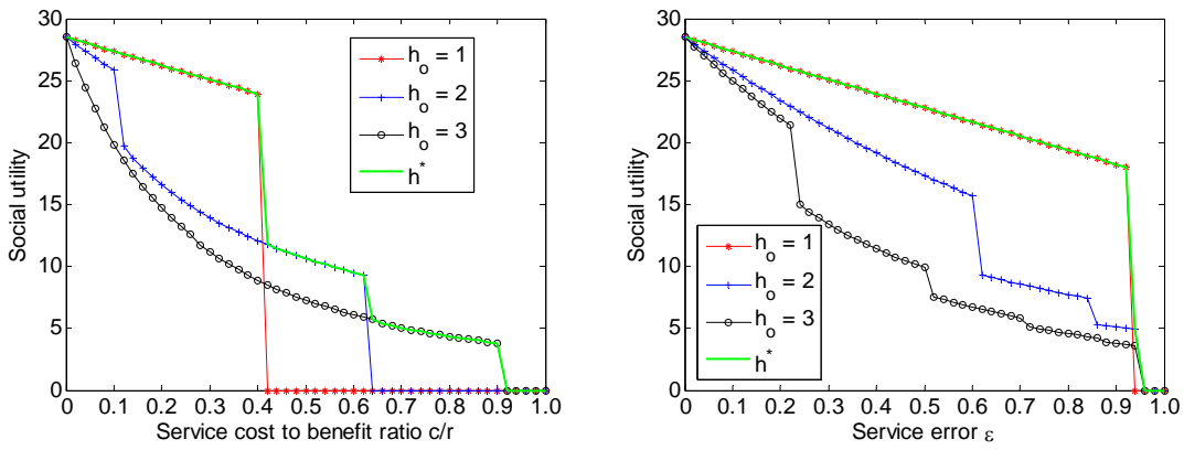
Figure 5. The protocols' performance against c/r and \epsilon .
