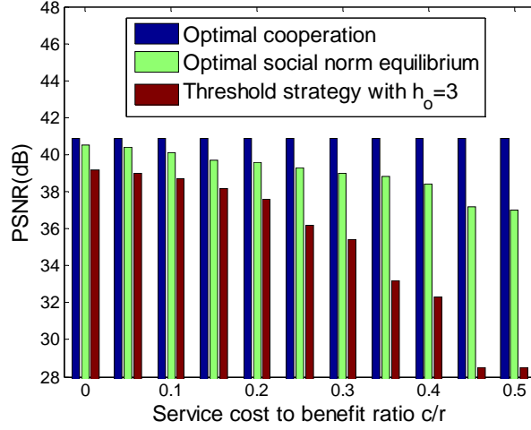
Figure 7. The PSNR of different protocols APPENDIX F
